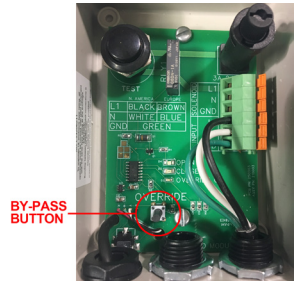
Figure 9 SOLENOID OVERRIDE Screen
